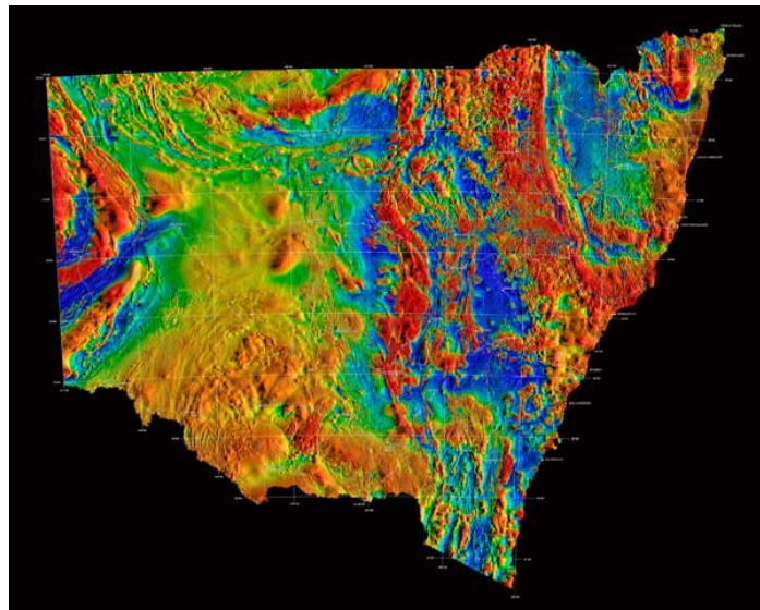
Geomagnetic map of the State of NSW Australia.
